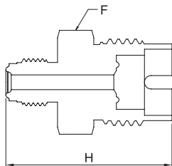
Face Seal Male
