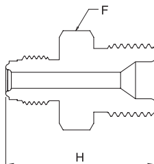
Faceseal Male
