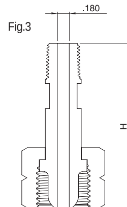
NPT Male
