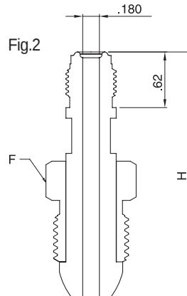
Facesal Male
